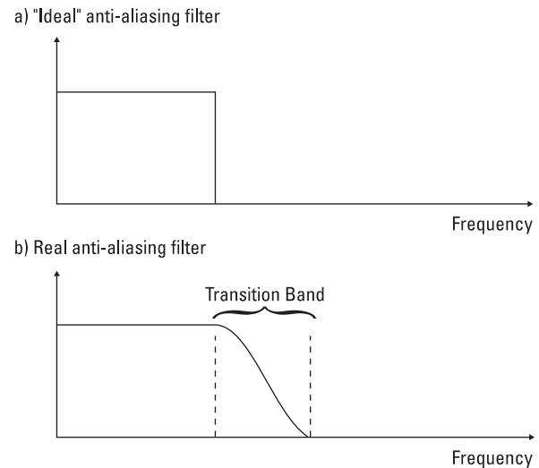
Figure 3.18 Actual anti-alias filters require higher sampling frequencies.
