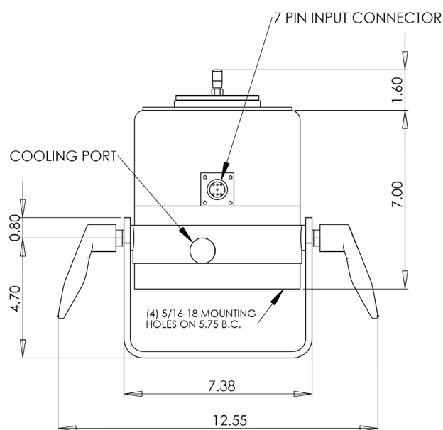
Modal 2075E - Front View
