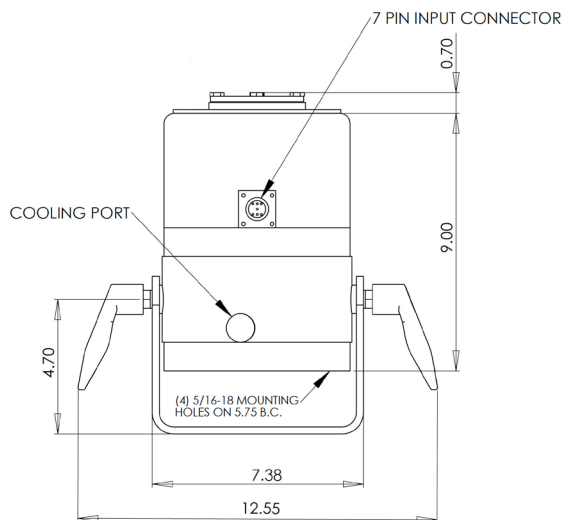
Model 2110E - Front View
