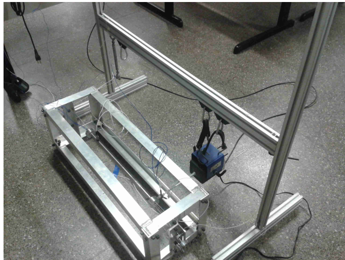
Figure 1. Test set - up for tests in x direction - air environment.
