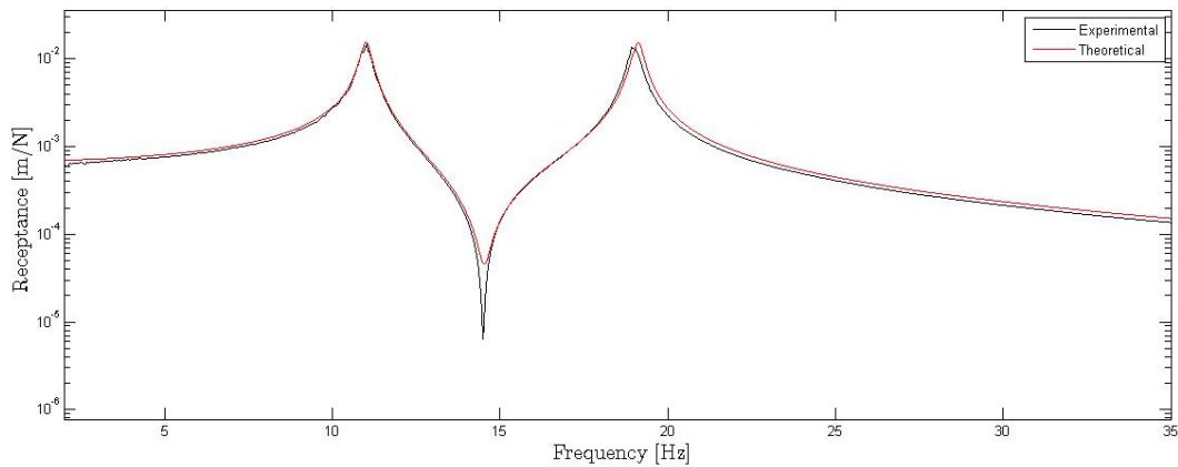
Figure 13. Experimental and theoretical FRFs in x coordinate in air - environment.
